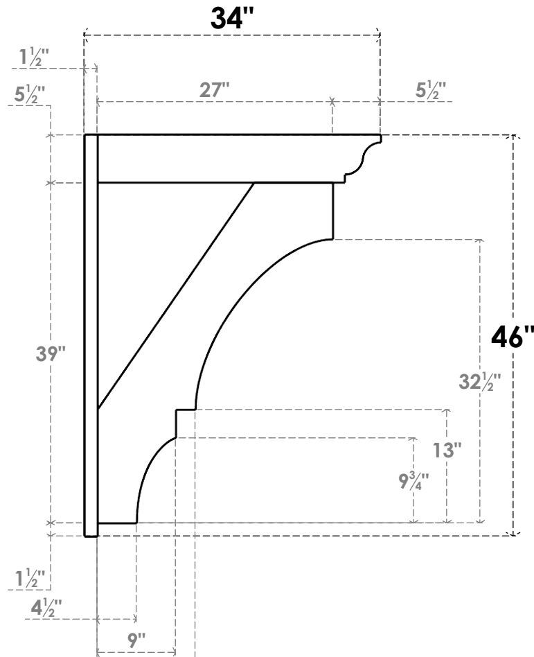
SIDE PROFILE
